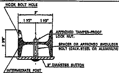
REFLECTOR MOUNT DETAIL PLAN VIEW
