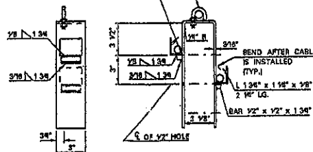
CROSSOVER END POST CAP ELEVATION VIEW
