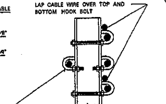
DETAIL "A" CENTER POST INTERMEDIATE ANCHORAGE SECTION
