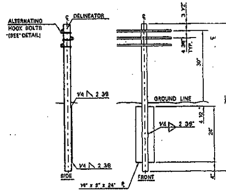
DOUBLE FACE CABLE GUARDRAIL INTERMEDIATE POST
