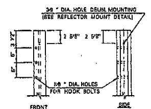
DOUBLE FACE CABLE GUARDRAIL POST HOLE PLACEMENT DETAIL INTERMEDIATE POST
