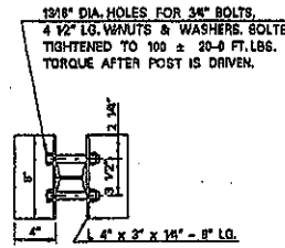
SECTION A-A BEARING PLATE
