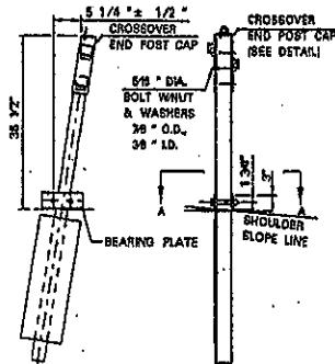
CROSSOVER END POST DOUBLE FACE
