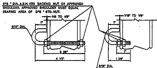
HOOK BOLT (ALTERNATES)
