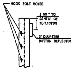
REFLECTOR MOUNT DETAIL ELEVATION VIEW
