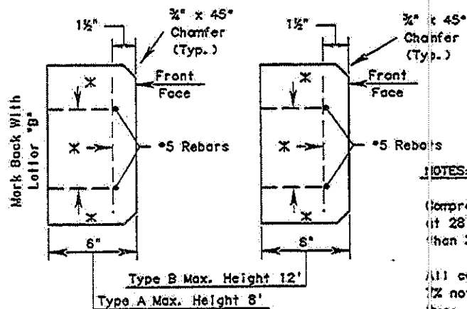
END VIEW
