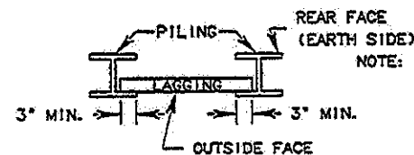
DETAIL 'A-A'
