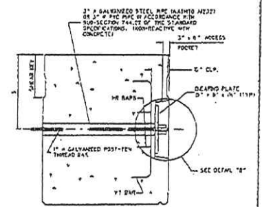
ACCESS POCKET END POST-TENSIONING BAR
