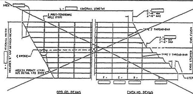
POST-TENSIONING BAR SPACING PLAN SHEET 1 OF 20
