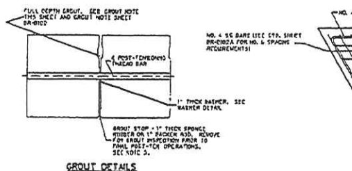
GROUT DETAILS
