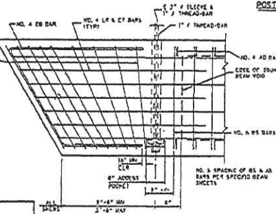
SHEAR REINFORCEMENT OCT.
