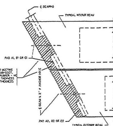
PLAN VIEW - BEARING PLACEMENT SKEWED BEAMS
