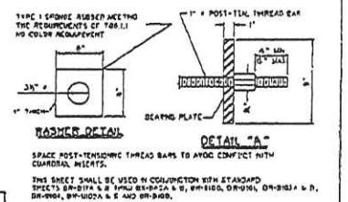
ACCESS POCKET END POST-TENSIONING BAR
