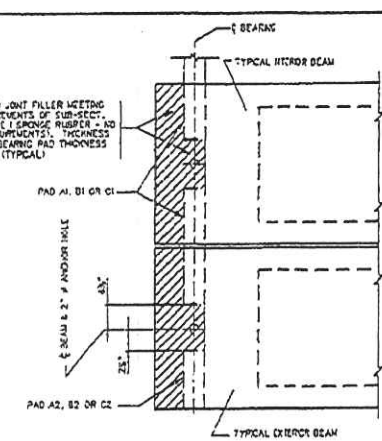
PLAN VIEW - BEARING PLACEMENT NORMAL BEAMS
