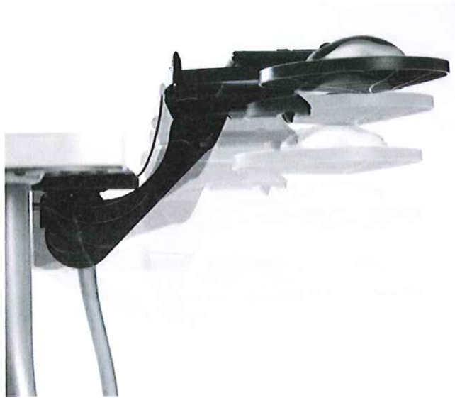
Adjusts through its entire range – 3.5" above the track and 5" below the track – and directly adjacent to the worksurface to help keep work within a neutral reach zone.
