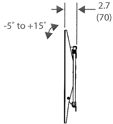
MOUNTING PROFILE
