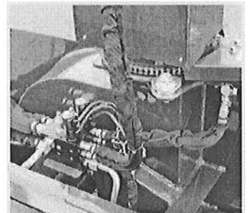
Hydraulic control valve with electric solenoid to control chute functions with built-in pressure relief system eliminating the need for shear pins.
