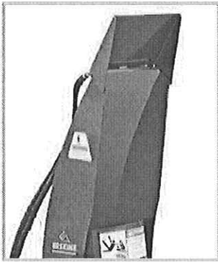
Hydraulic chute rotation and deflector – eliminates metal-to-metal contact between blower and rotating chute base preventing freeze up.
