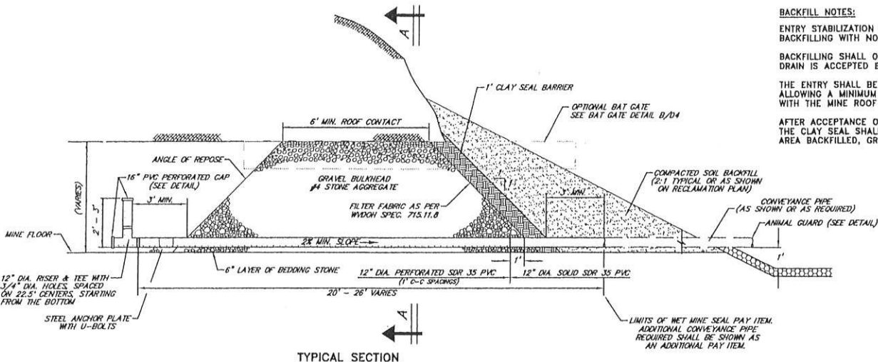
TYPICAL SECTION
