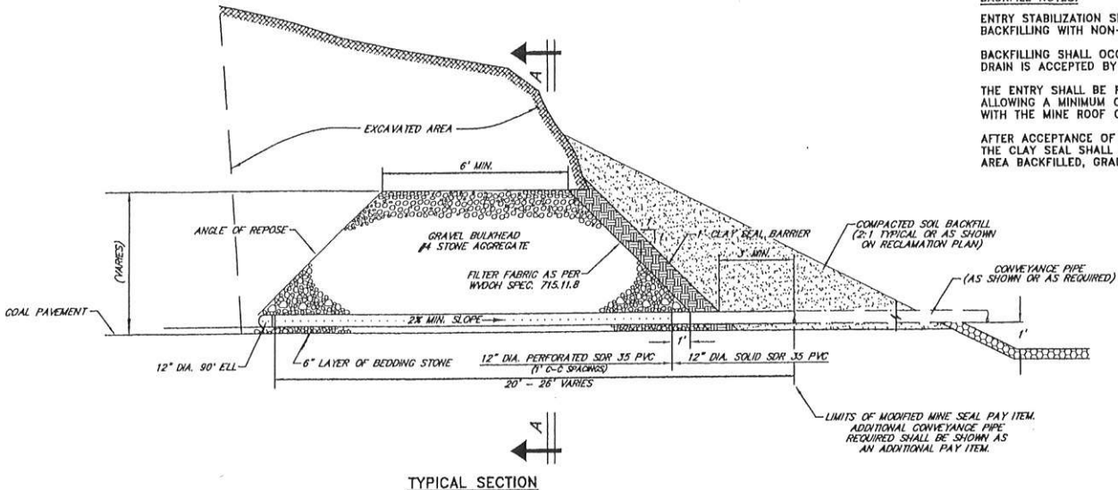
TYPICAL SECTION
