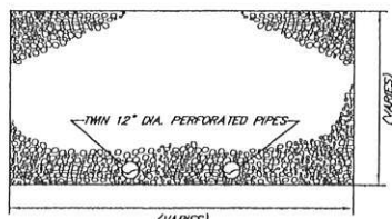
SECTION A-A STONE BULKHEAD
