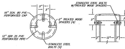
PERFORATED CAP DETAIL
