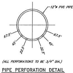
PIPE PERFORATION DETAIL
