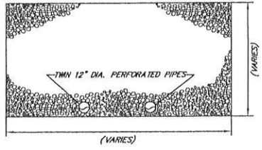
SECTION A-A STONE BULKHEAD
