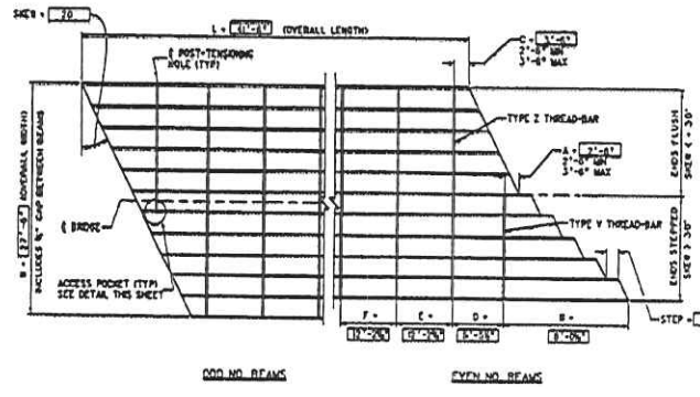
POST-TENSIONING BAR SPACING PLAN SHEET > = 20'
