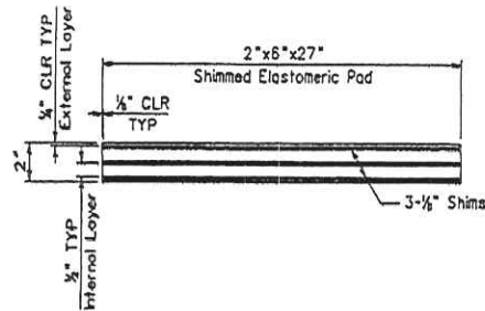
SHIMMED ELASTOMERIC BEARING PAD
