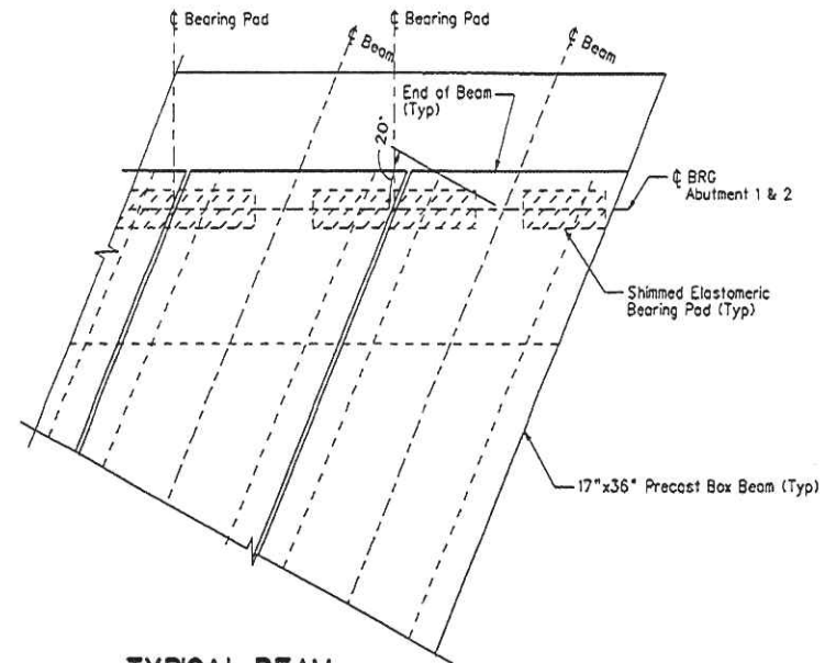
TYPICAL BEAM BEARING DETAIL
