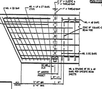
SHEAR REINFORCEMENT DETAIL BEAMS WITH ACCESS POCKETS
