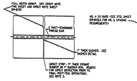
GROUT DETAILS
