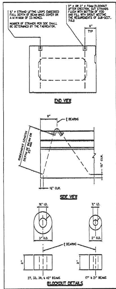
LIFTING DETAILS
