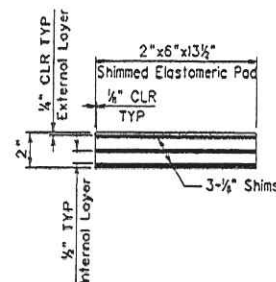
SHIMMED ELASTOMERIC BEARING PAD @ ABUTMENT 1 & 2
