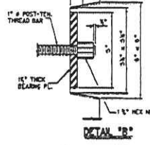
REINFORCING DETAILS @ DIAPHRAGM EXTERIOR BEAM @ POCKETS ONLY
