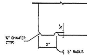
DRP GROOVE DETAIL EXTERIOR BEAMS
