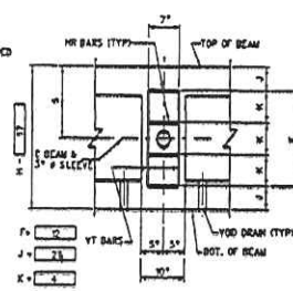
REINFORCING DETAILS @ DIAPHRAGM EXTERIOR BEAM @ POCKETS ONLY
