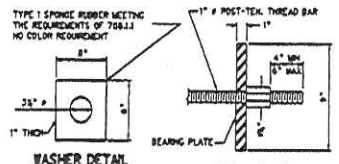
WASHER DETAIL
