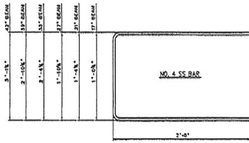
END BEARING DETAIL WITH BACKFALL
