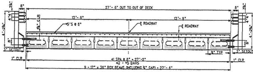
TYPICAL BRIDGE SECTION
