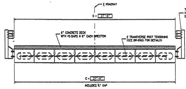
TYPICAL CROSS-SECTION WITH GUARDRAIL
