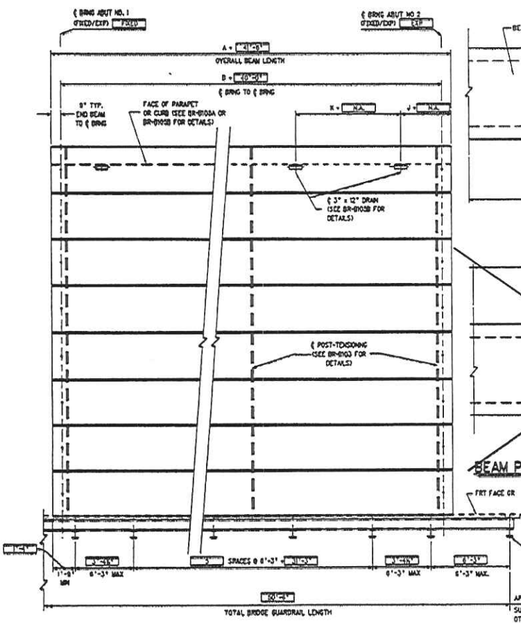
DECK PLAN VIEW
