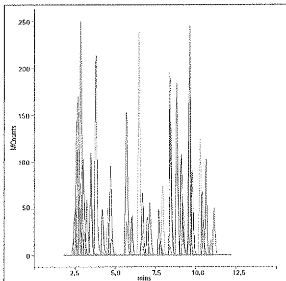
Varian 325-MS LC/MS with SRM transitions offers high quality quantification with more than 10 data points per peak and an analysis of 48 pesticides in less than 11 minutes.
