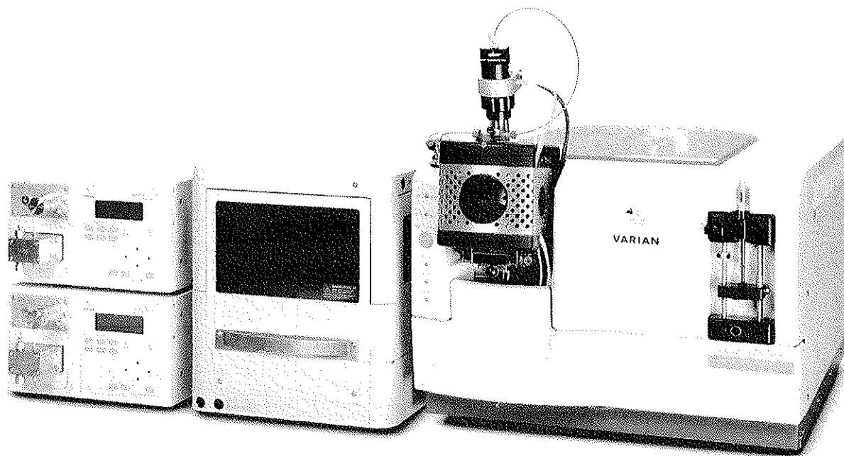
The standard configuration contains: 325-MS with vESI interface, 212-IC pumps and choice of autosampler (shown here with the 460-IC autosampler).
