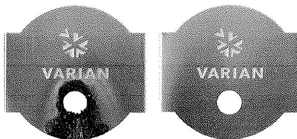
The complex, dirty matrix that accumulates on the spray shield (left) is easily removed. Cleaning the Gold Guard with a moist wipe restores the chemically resistant shield to its original condition (right).
