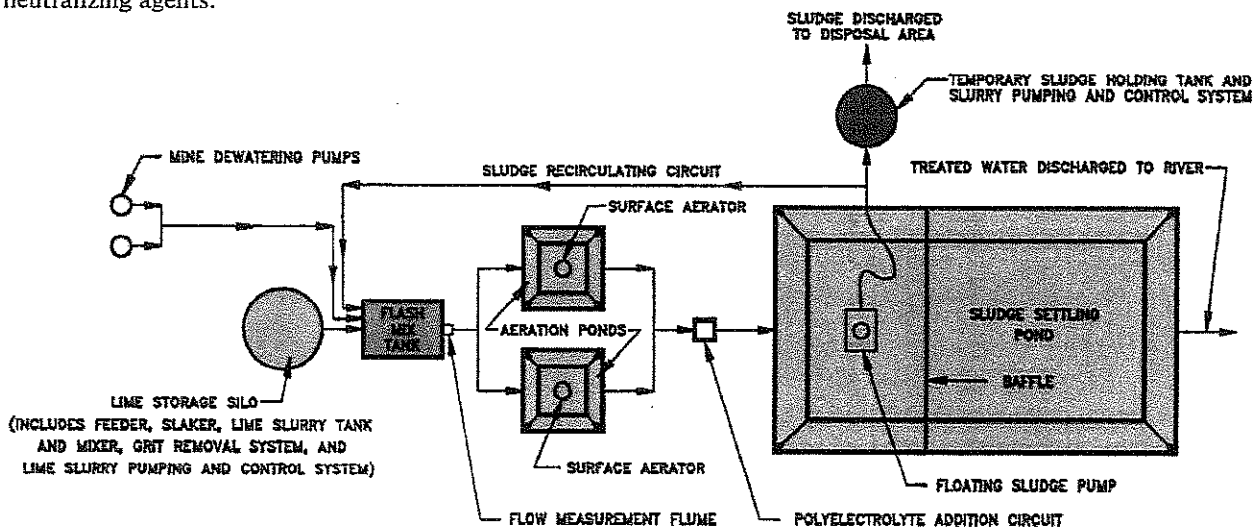
Schematic diagram of the 4-million-gallon per day acid mine drainage plant.
