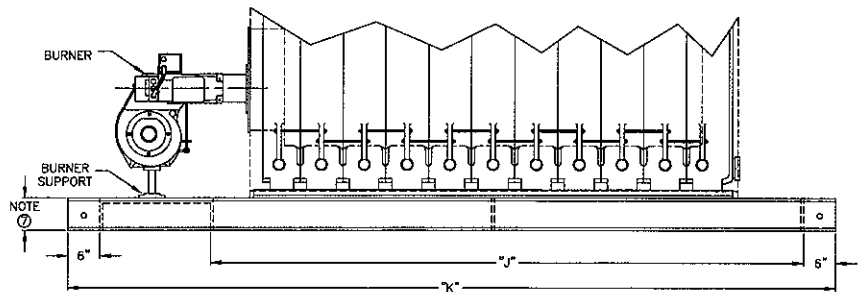
TYPICAL ASSEMBLY – SIDE VIEW
