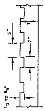
ALTERNATE SECTION B-B (SAVED RUMBLE STRIP)
