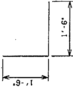
W501 - #5 BENT BARS
