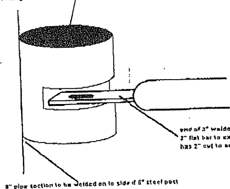
1/2" dia. X 6" long pipe section for lock housing, top of housing is welded on steel cap
