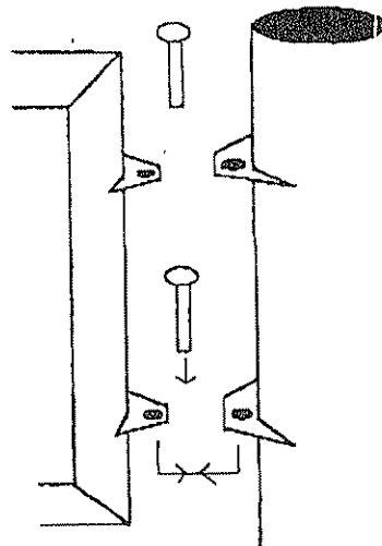
welded 1/2" steel flanges to vertical with 1" cut hole to align for 1" steel pin to insert. Pin will be secured to prevent removal after installation but allow free movement of gate.
