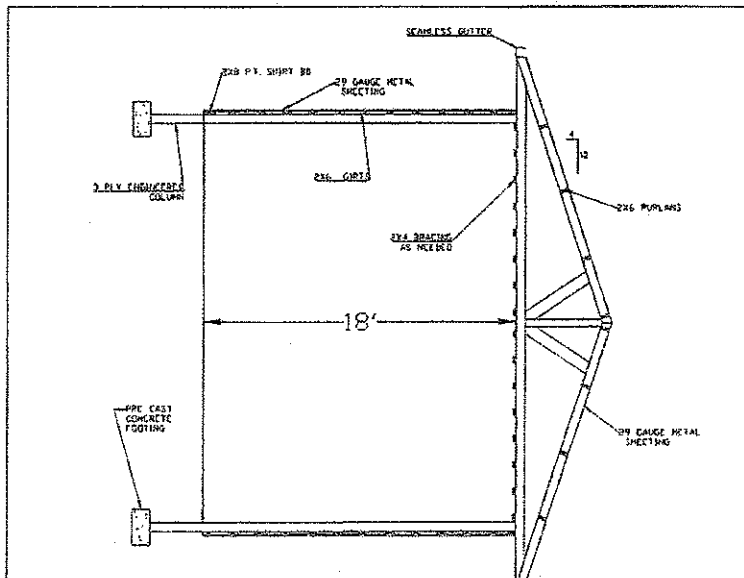
CROSS SECTION
