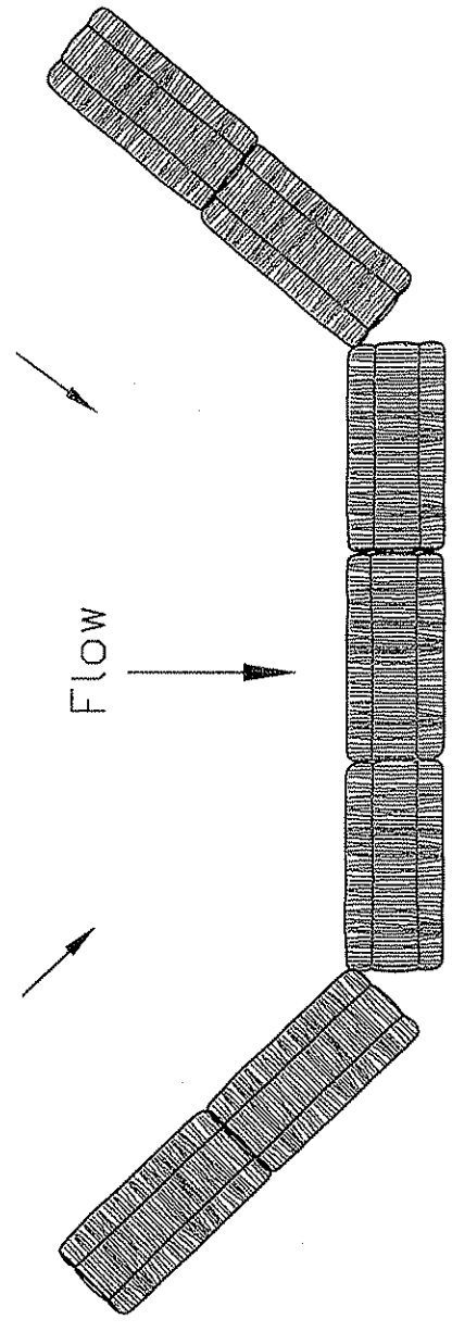
DESIGN TO FIT SITE CONDITIONS SEDIMENT BARRIER TOP VIEW
