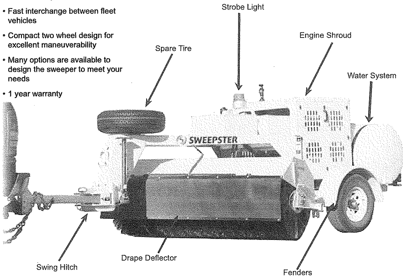
TBCP shown with optional spare tire, engine shroud, water system, drape deflector, strobe light, fenders & swing hitch.
