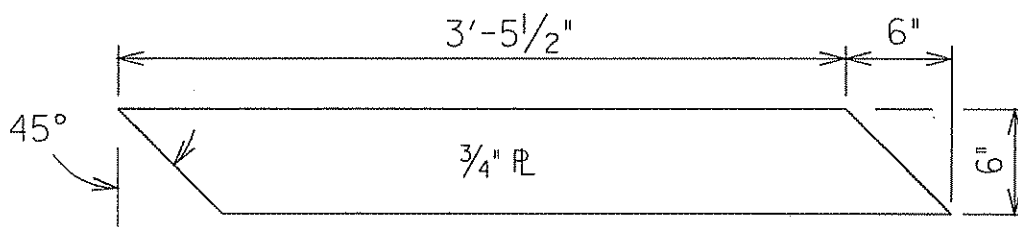
GALVANIZED 3/4" PLATE - MARK P2 ( 6 - Required )
