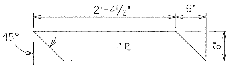
GALVANIZED 1" PLATE - MARK P1 ( 6 - Required )
