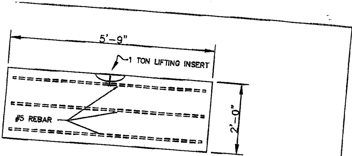
FRONT ELEVATION
