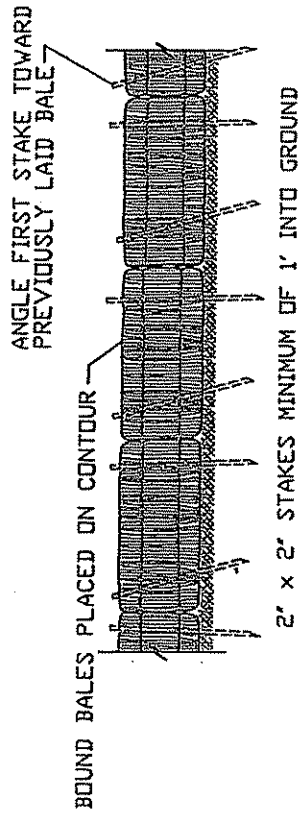
ANCHORING DETAIL
