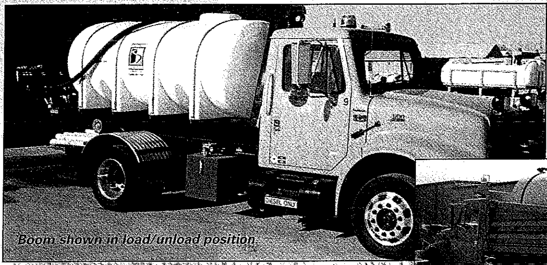
Boom custom built for removal during loading onto Hook Lift™.
