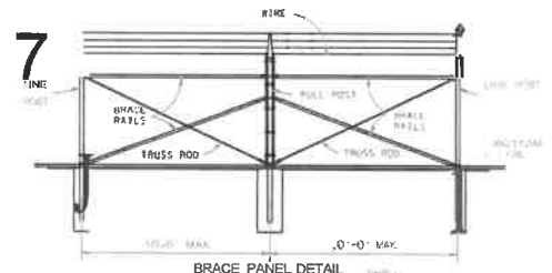
BRACE PANEL DETAIL NO SCALE
