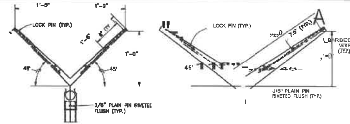
CORNER POST
