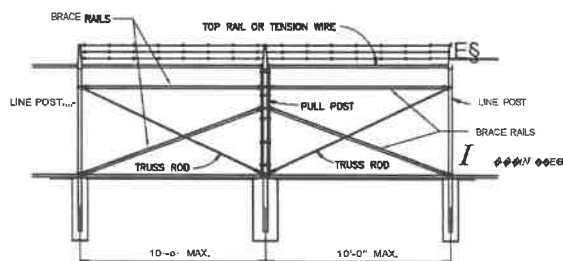
1.8 BRACE PANEL DETAIL 1/4\"/>
