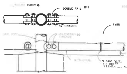
BOTTOM RAIL DETAILS
