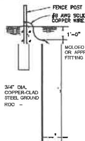
1.5 GROUNDING DETAIL 1/4\"/>
