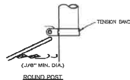
1.2 TENSION BAND DETAIL 1/4\"/>
