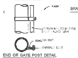
END OR GATE POST DETAIL
