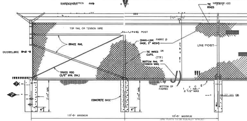
1.1 CHAIN-LINK SECURITY FENCE DETAIL 1/4\"/>
