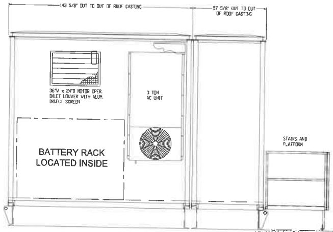
"B" END WALL
