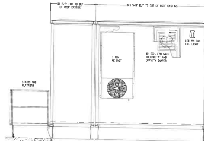
"D" END WALL
