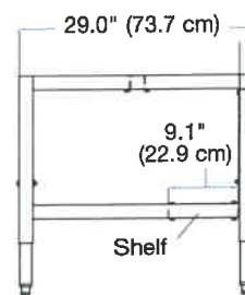
SIDE
