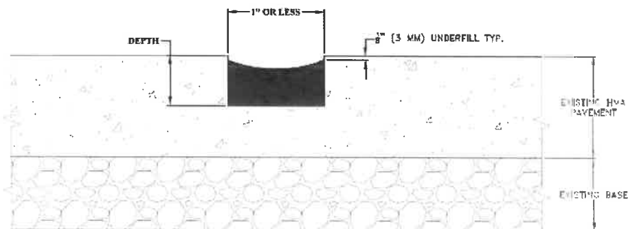
CRACK REPAIR IN FLEXIBLE PAVEMENT
