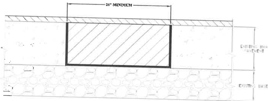
FULL DEPTH CRACK REPAIR IN FLEXIBLE PAVEMENT
