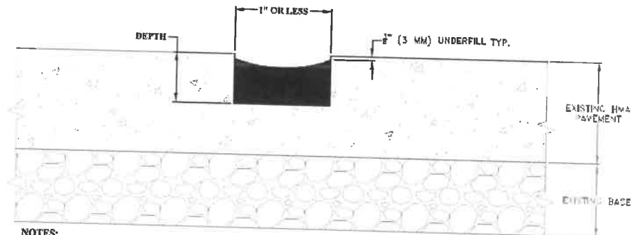
CRACK REPAIR IN FLEXIBLE PAVEMENT
