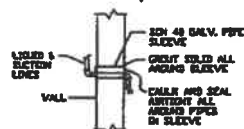
REFRIGERANT LINES WALL PENETRATION DETAIL AS SHOWN
