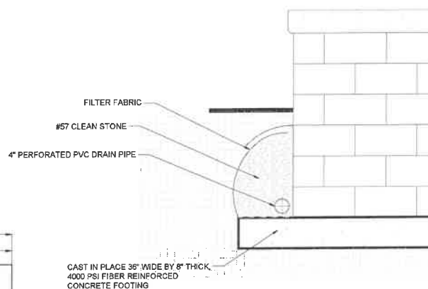
FOOTER DRAIN DETAILS SCALE 1-1/2" = 1'
