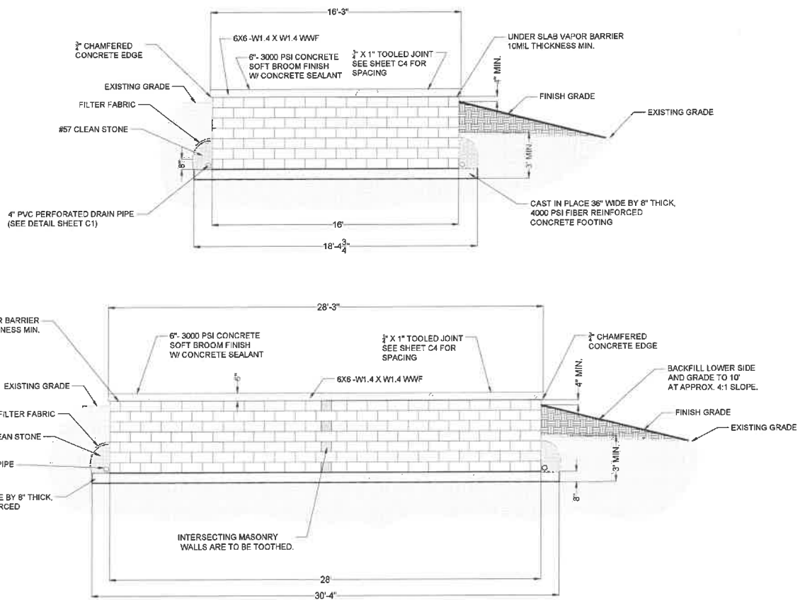
FOUNDATION PLAN
