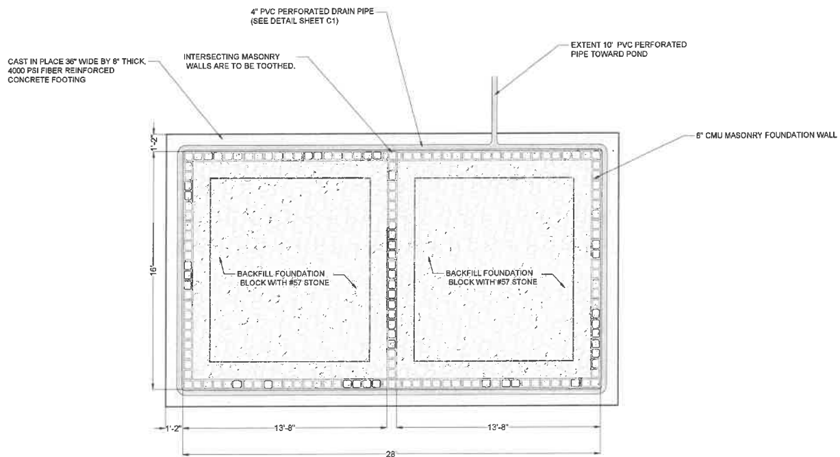
FOUNDATION PLAN SCALE 1" = 1'
