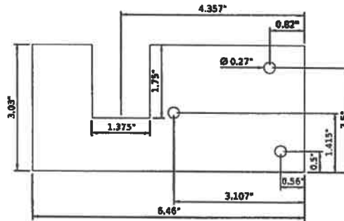
STEEL DECK CLIP FOR 1-3/8" FLANGE
