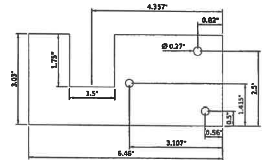
STEEL DECK CLIP FOR 1-1/2" FLANGE
