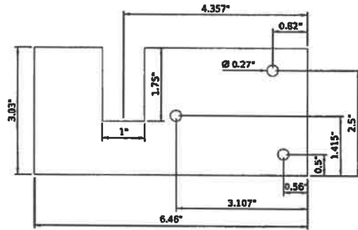
STEEL DECK CLIP FOR 1" FLANGE
