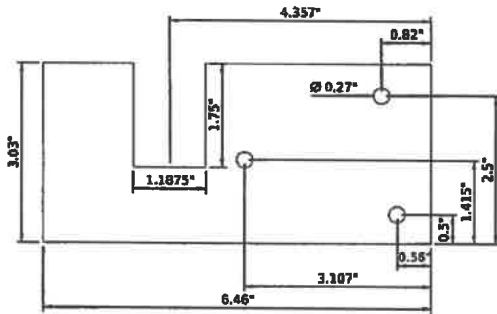
STEEL DECK CLIP FOR 1-3/16" FLANGE
