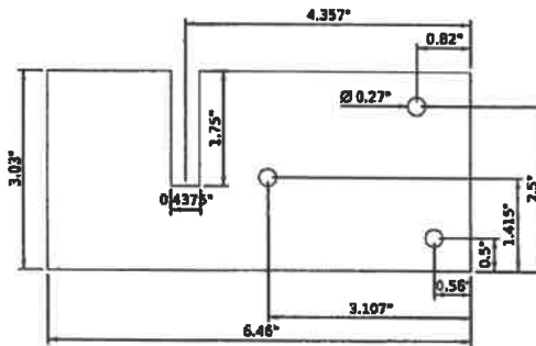
STEEL DECK CLIP FOR 7/16" FLANGE
