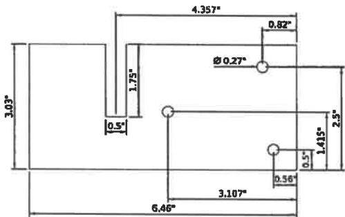
STEEL DECK CLIP FOR 1/2" FLANGE
