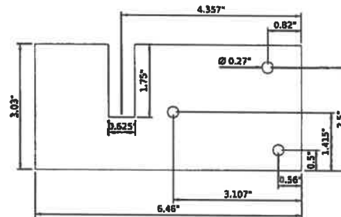
STEEL DECK CLIP FOR 5/8" FLANGE
