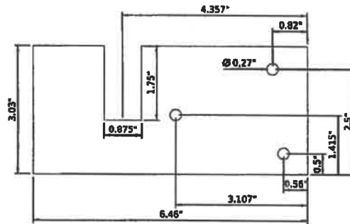
STEEL DECK CLIP FOR 7/8" FLANGE
