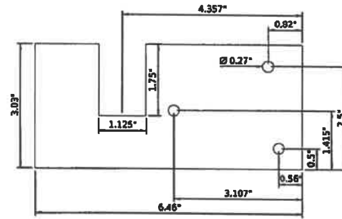
STEEL DECK CLIP FOR 1-1/8" FLANGE
