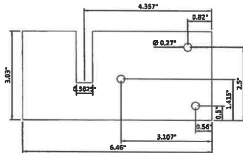
STEEL DECK CLIP FOR 9/16" FLANGE
