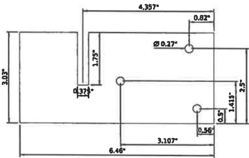
STEEL DECK CLIP FOR 3/8" FLANGE
