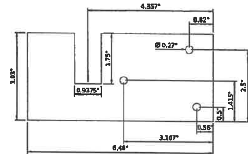
STEEL DECK CLIP FOR 15/16" FLANGE
