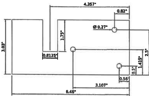
STEEL DECK CLIP FOR 13/16" FLANGE
