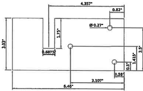
STEEL DECK CLIP FOR 11/16" FLANGE
