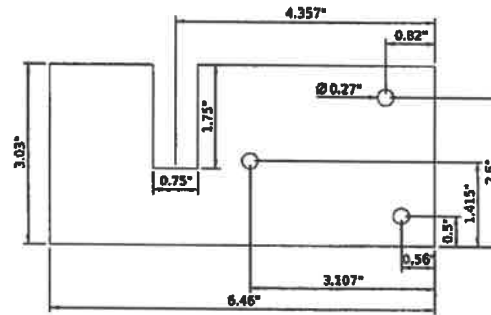
STEEL DECK CLIP FOR 3/4" FLANGE
