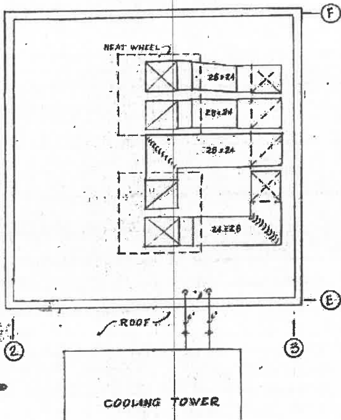
PENTHOUSE ROOF PLAN
