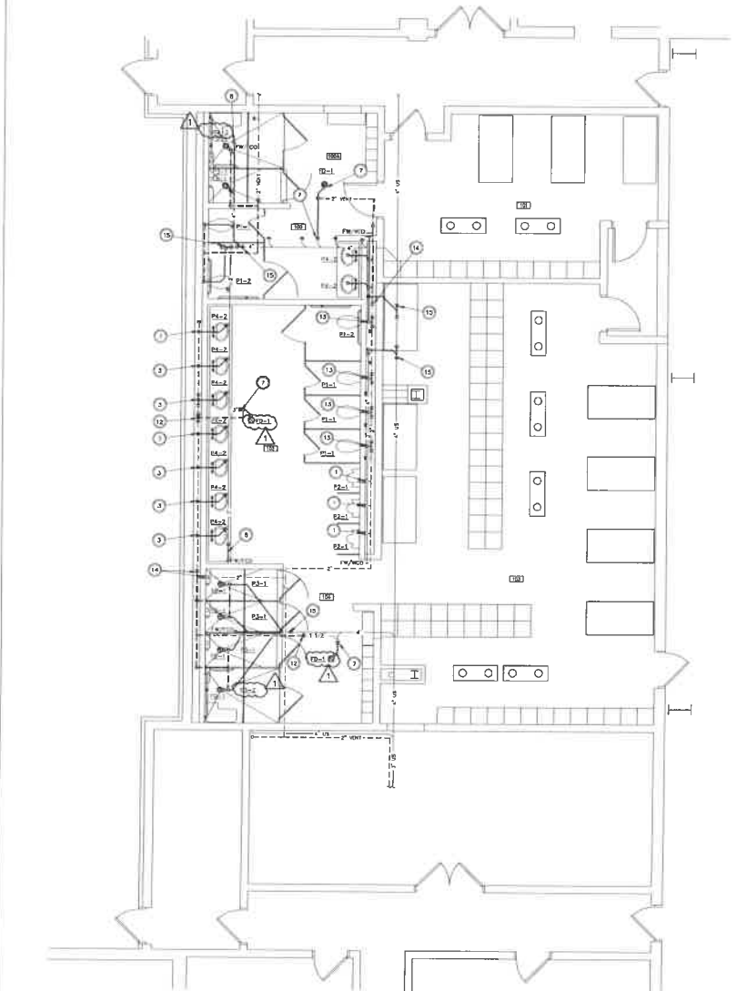
NEW WORK - FIRST FLOOR MEN'S & WOMEN'S LATRINE/SHOWERS/LOCKER ROOMS - SANITARY
