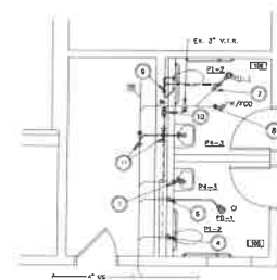
NEW WORK - FIRST FLOOR LATRINE/SHOWER - SANITARY
