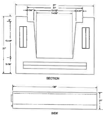
TRENCH DRAIN DETAIL NOT TO SCALE
