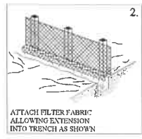
BUILDING SILT FENCE - STEP BY STEP PROCEDURE NOT TO SCALE
