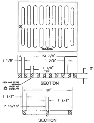
TRENCH GRATE DETAIL NOT TO SCALE
