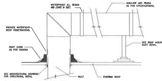
DUCT ROOF PENETRATION AND SUPPORT DETAIL N.T.S.
