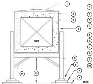
ROOF MOUNTED DUCT DETAIL NO SCALE
