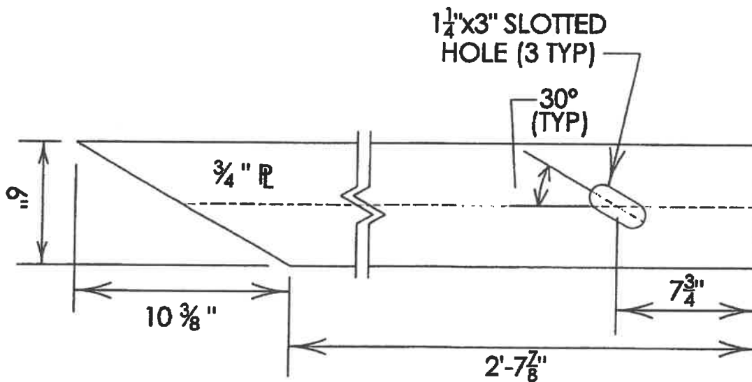
GALVANIZED \frac{3}{4}" PLATE - MARK M5 2 Required
