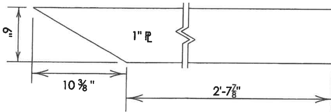
GALVANIZED 1" PLATE - MARK M4 2 Required
