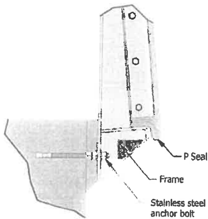
Invert Seal
