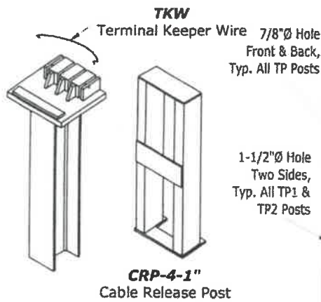
AP-4 Anchor Post
